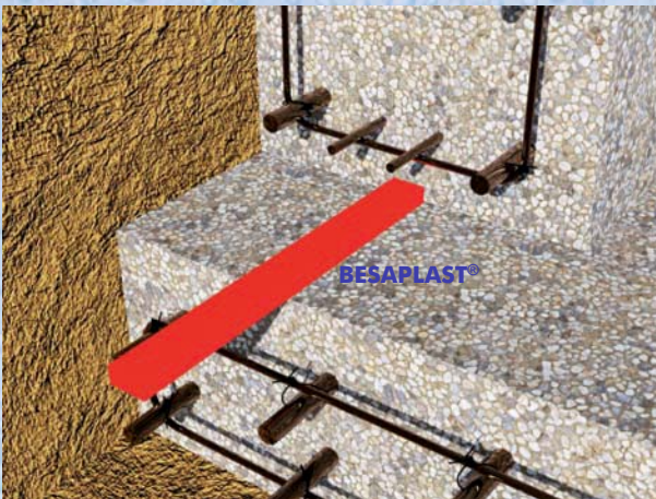
Quellband / swelling rubber
