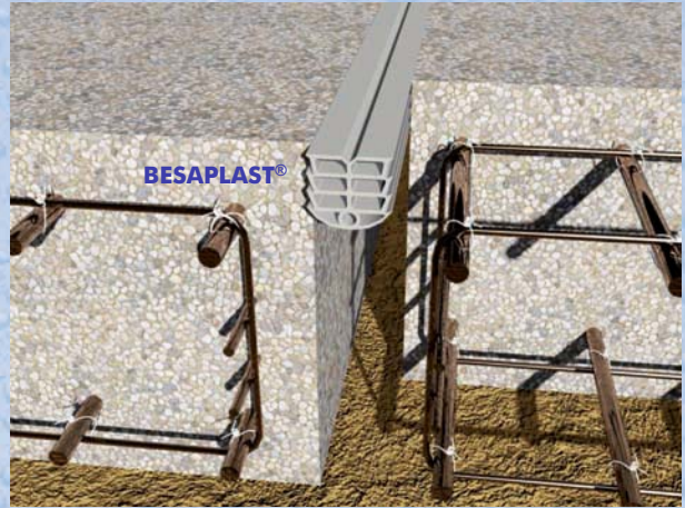
Klemmprofile / compression profiles
