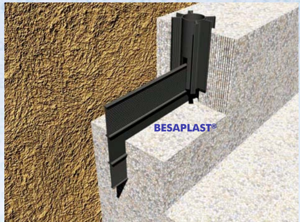
Schwindrohr / shrinkage tube
